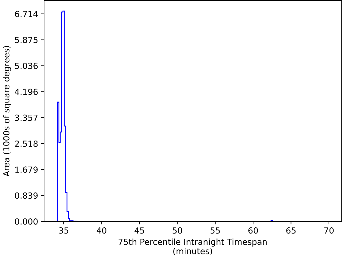
too_elab_2yr_r128_d2_griz_v3.4_10yrs All sky all bands: 75th Percentile Intranight Timespan
