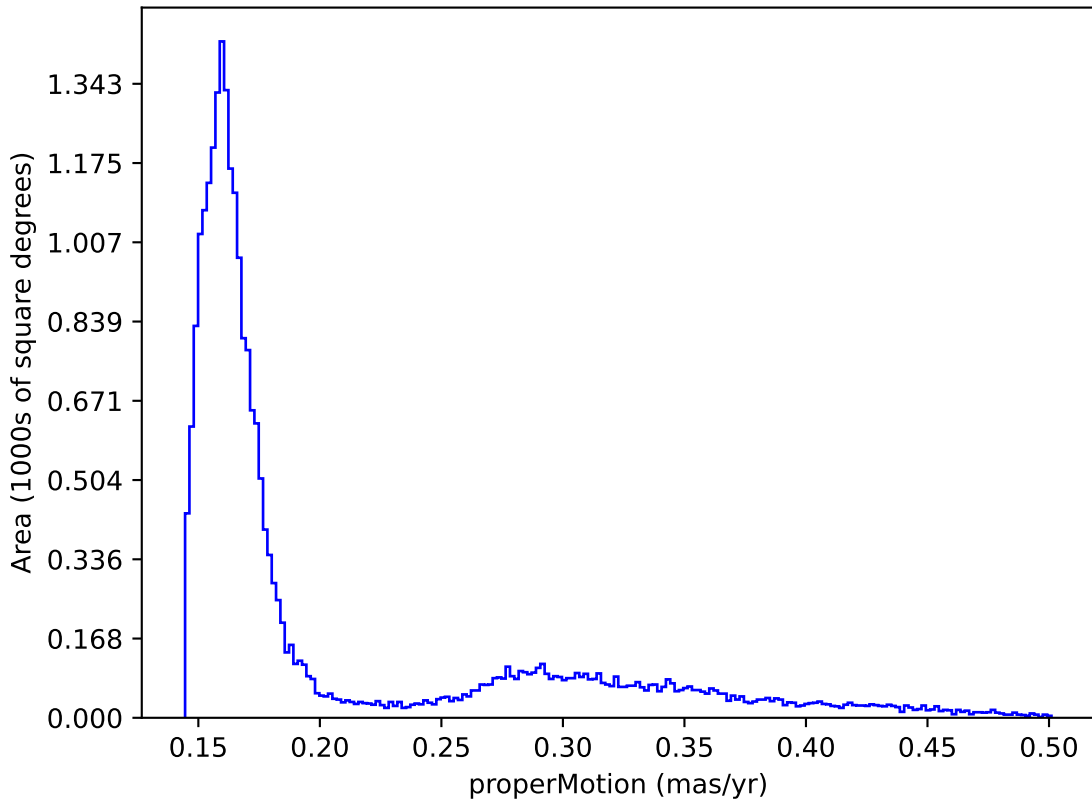
too_elab_2yr_r128_d2_griz_v3.4_10yrs : properMotion
