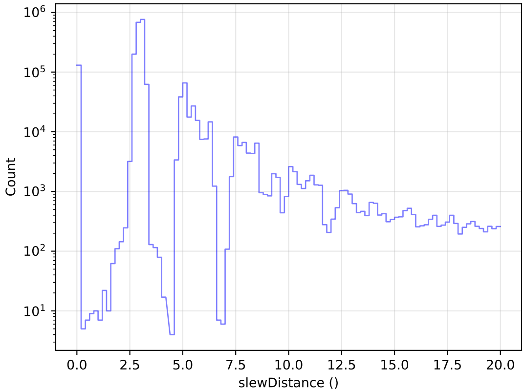
too_elab_2yr_r128_d2_griz_v3.4_10yrs All visits: Zoom Slew Distance Histogram
