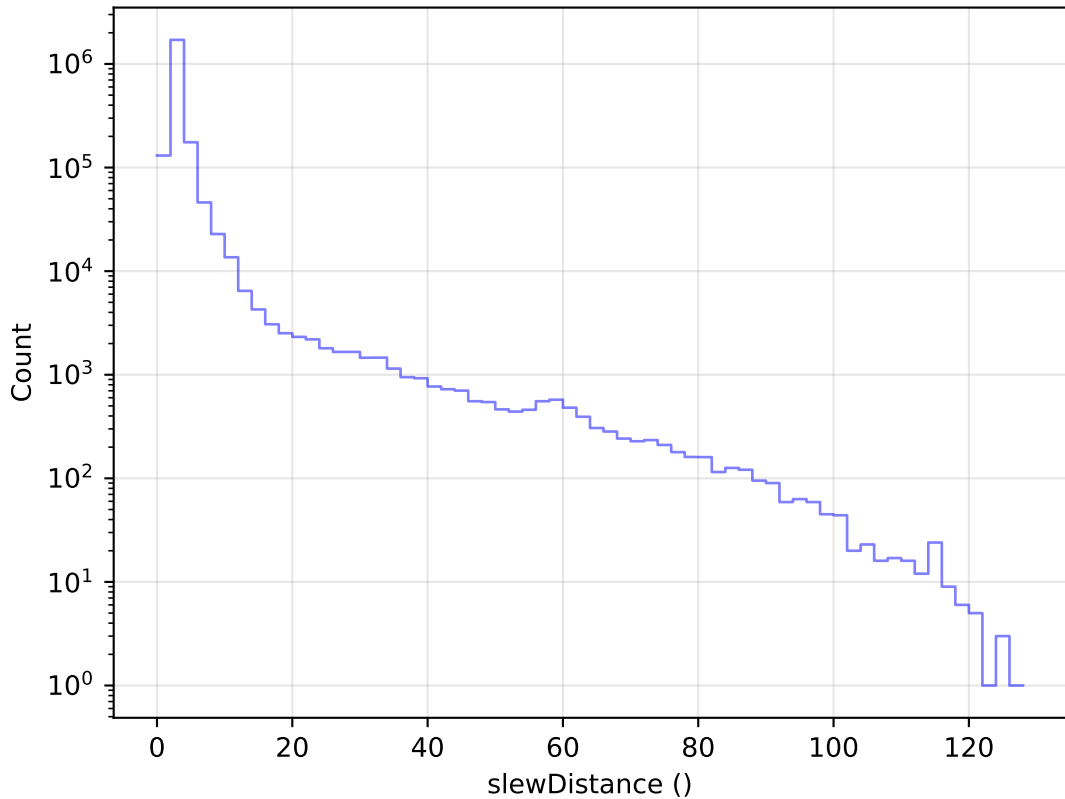
too_elab_2yr_r128_d2_griz_v3.4_10yrs All visits: Slew Distance Histogram
