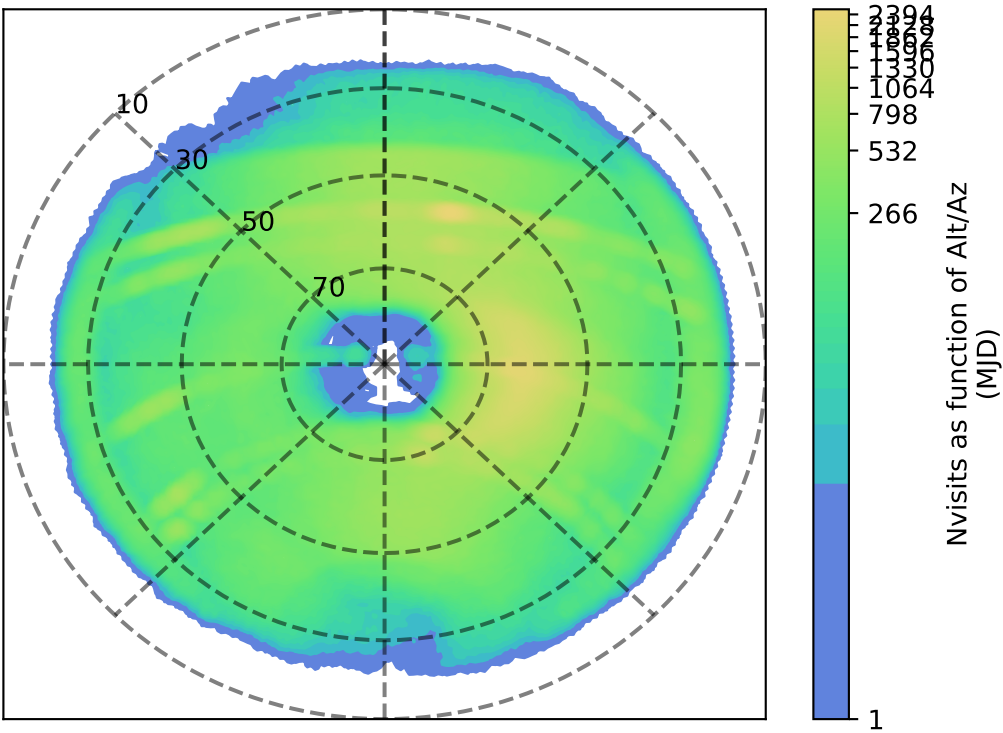
too_elab_2yr_r128_d2_griz_v3.4_10yrs z: Nvisits as function of Alt/Az
