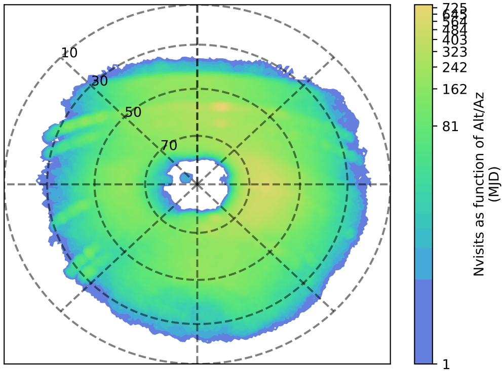
too_elab_2yr_r128_d2_griz_v3.4_10yrs u: Nvisits as function of Alt/Az
