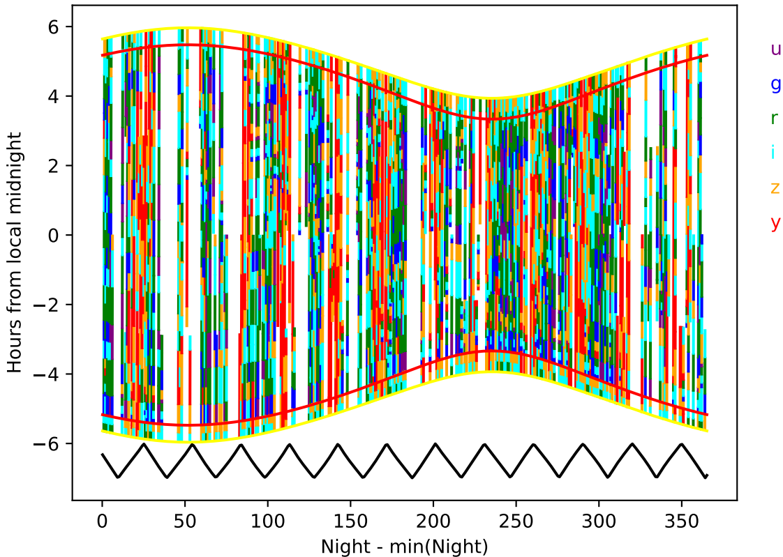
too_elab_2yr_r128_d2_griz_v3.4_10yrs year 7-8: Hourglass
