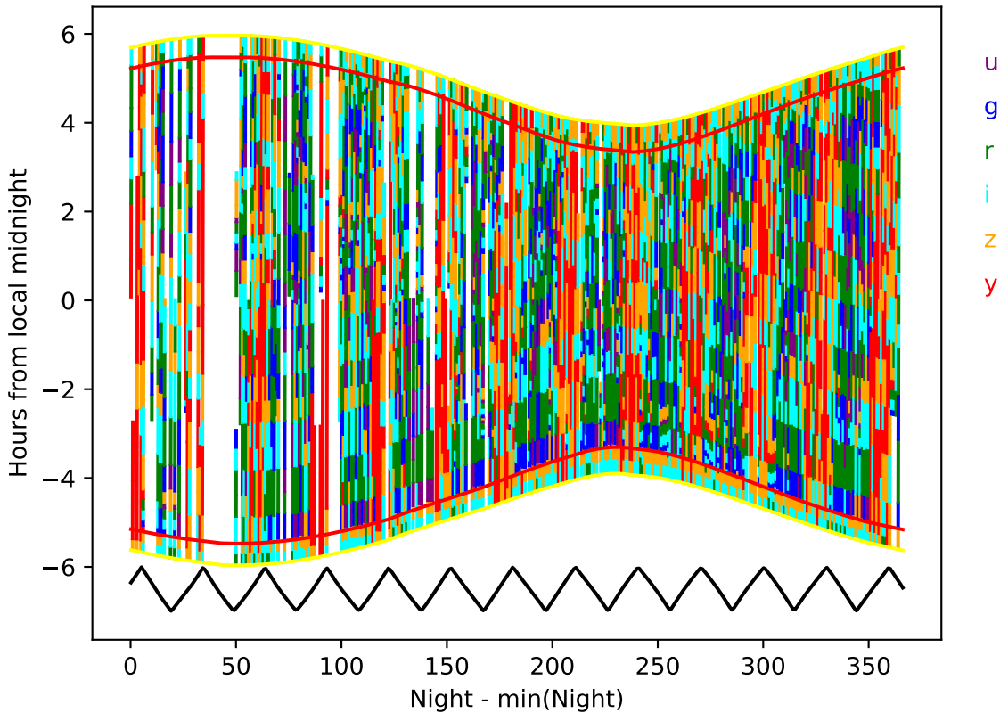
too_elab_2yr_r128_d2_griz_v3.4_10yrs year 6-7: Hourglass
