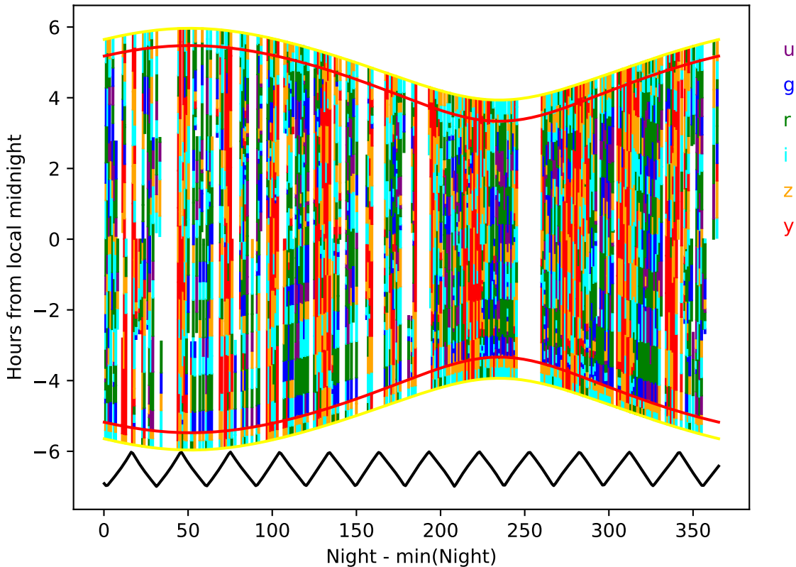
too_elab_2yr_r128_d2_griz_v3.4_10yrs year 5-6: Hourglass
