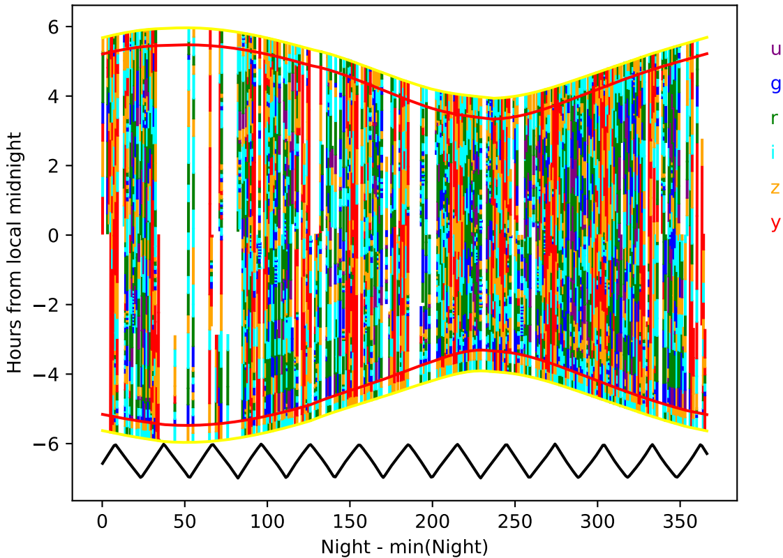
too_elab_2yr_r128_d2_griz_v3.4_10yrs year 3-4: Hourglass
