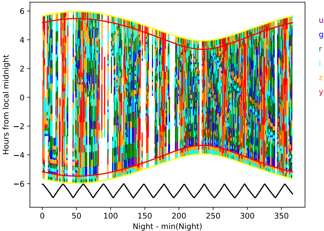
too_elab_2yr_r128_d2_griz_v3.4_10yrs year 1-2: Hourglass
