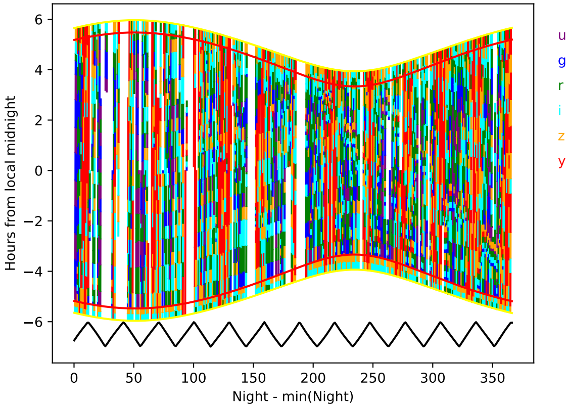
too_elab_2yr_r128_d2_griz_v3.4_10yrs year 0-1: Hourglass
