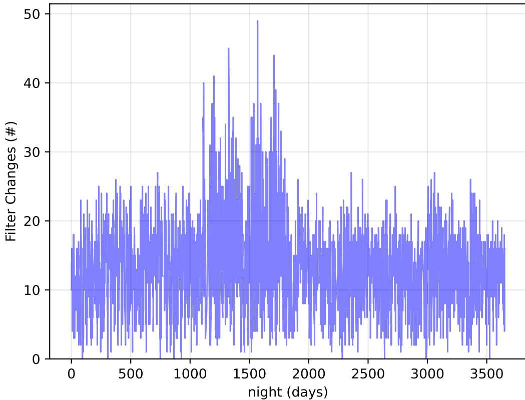
too_elab_2yr_r128_d2_griz_v3.4_10yrs : Filter Changes
