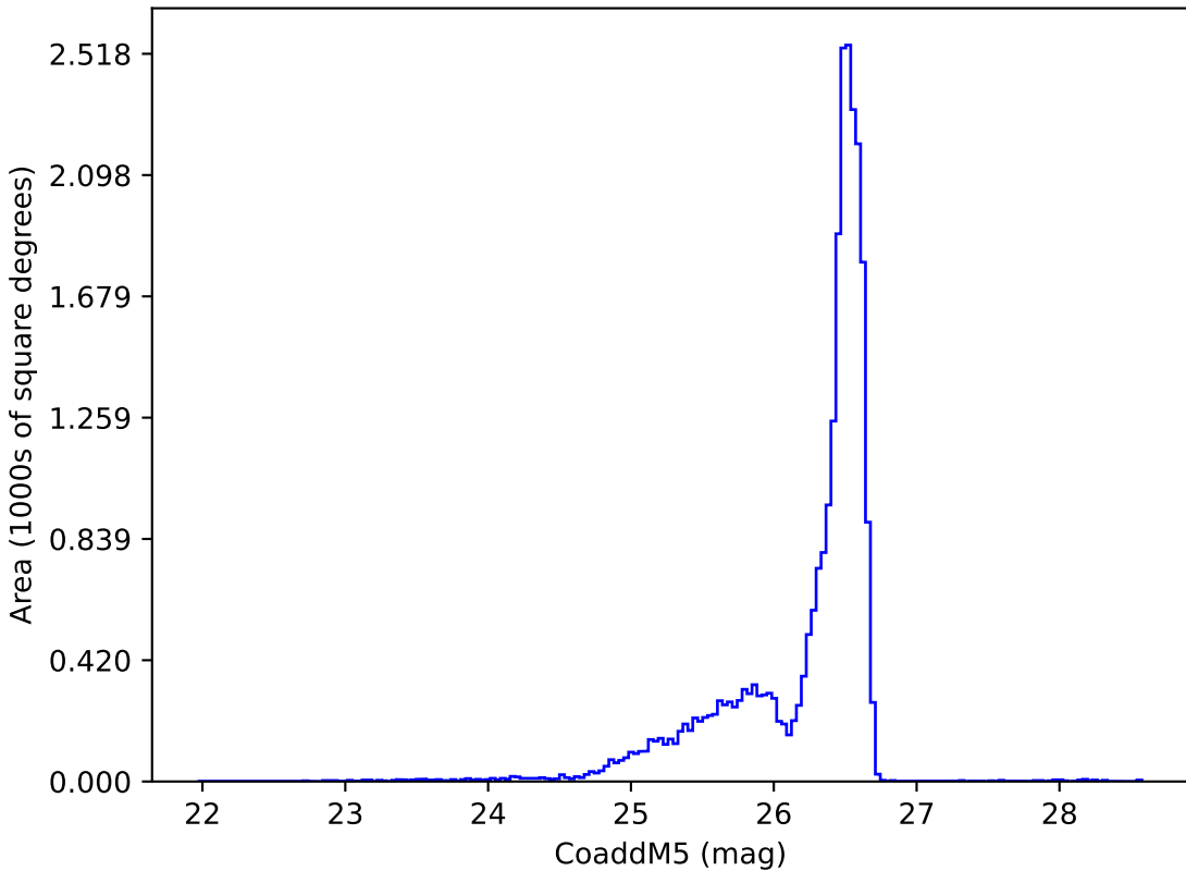
too_elab_2yr_r128_d2_griz_v3.4_10yrs i: CoaddM5
