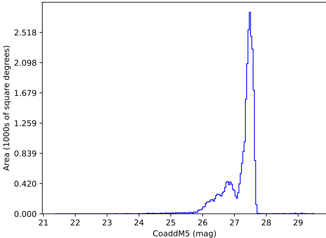
too_elab_2yr_r128_d2_griz_v3.4_10yrs : CoaddM5
