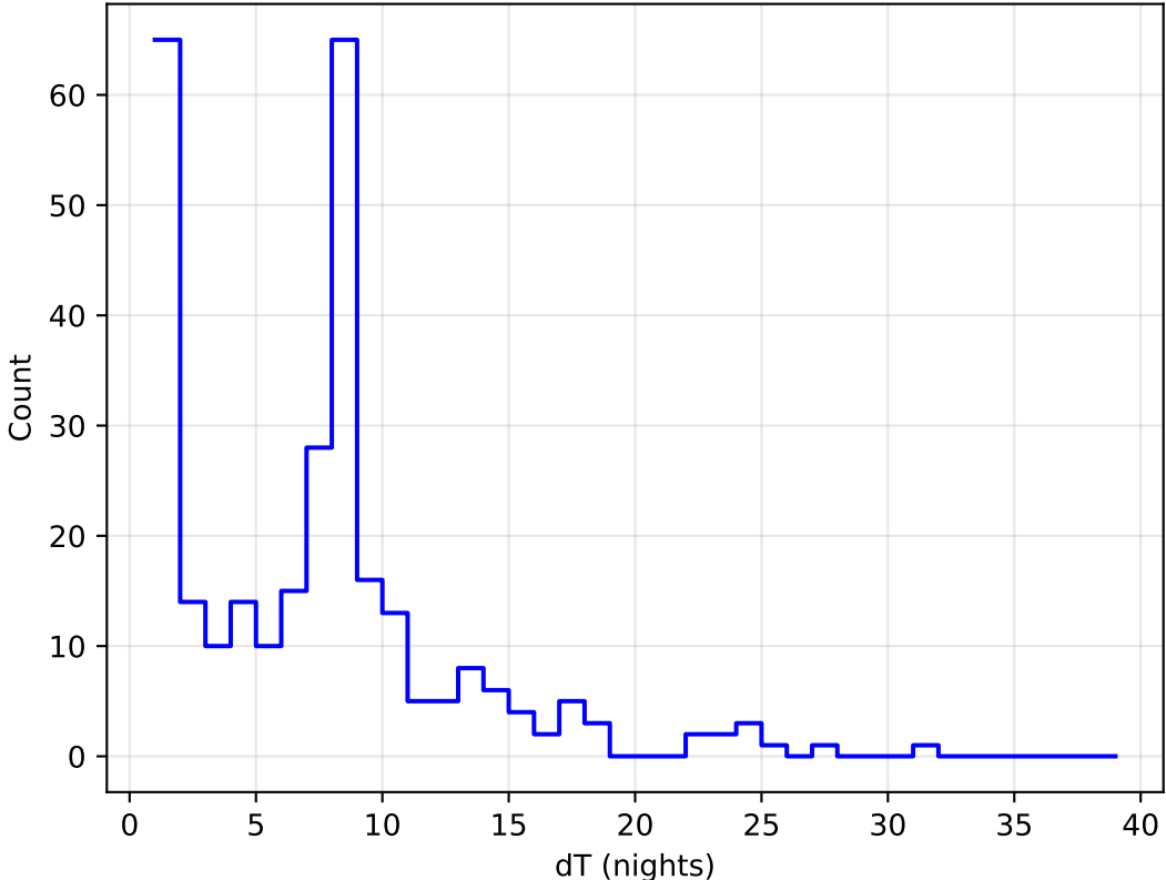
too_elab_2yr_r128_d2_griz_v3.4_10yrs all bands: DD:XMM_LSS Delta Nights Histogram
