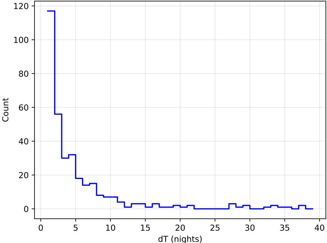
too_elab_2yr_r128_d2_griz_v3.4_10yrs all bands: DD:WFD Delta Nights Histogram
