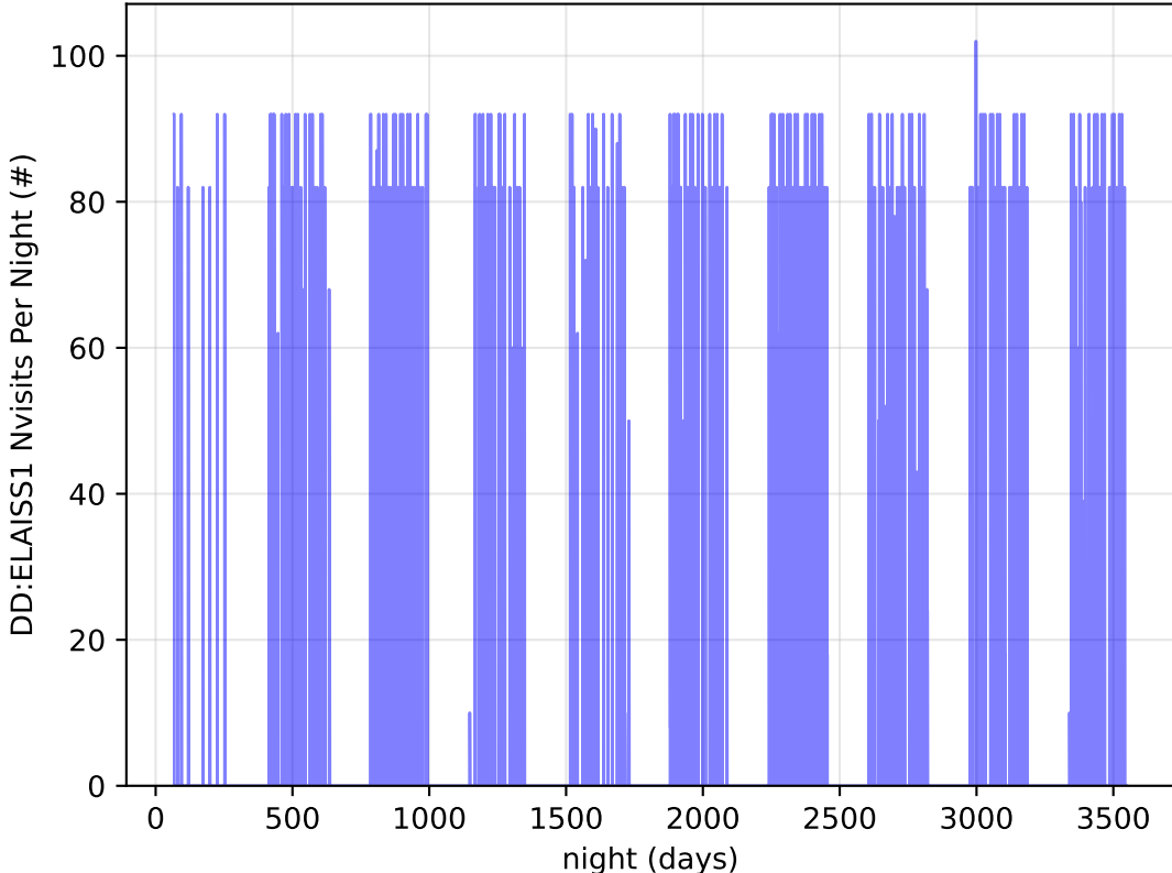
too_elab_2yr_r128_d2_griz_v3.4_10yrs all bands: DD:ELAISS1 Nvisits Per Night
