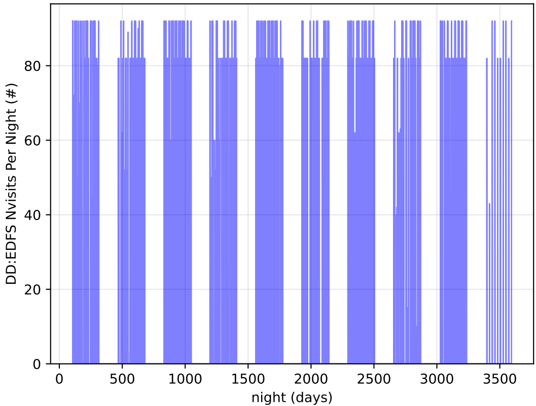
too_elab_2yr_r128_d2_griz_v3.4_10yrs all bands: DD:EDFS Nvisits Per Night
