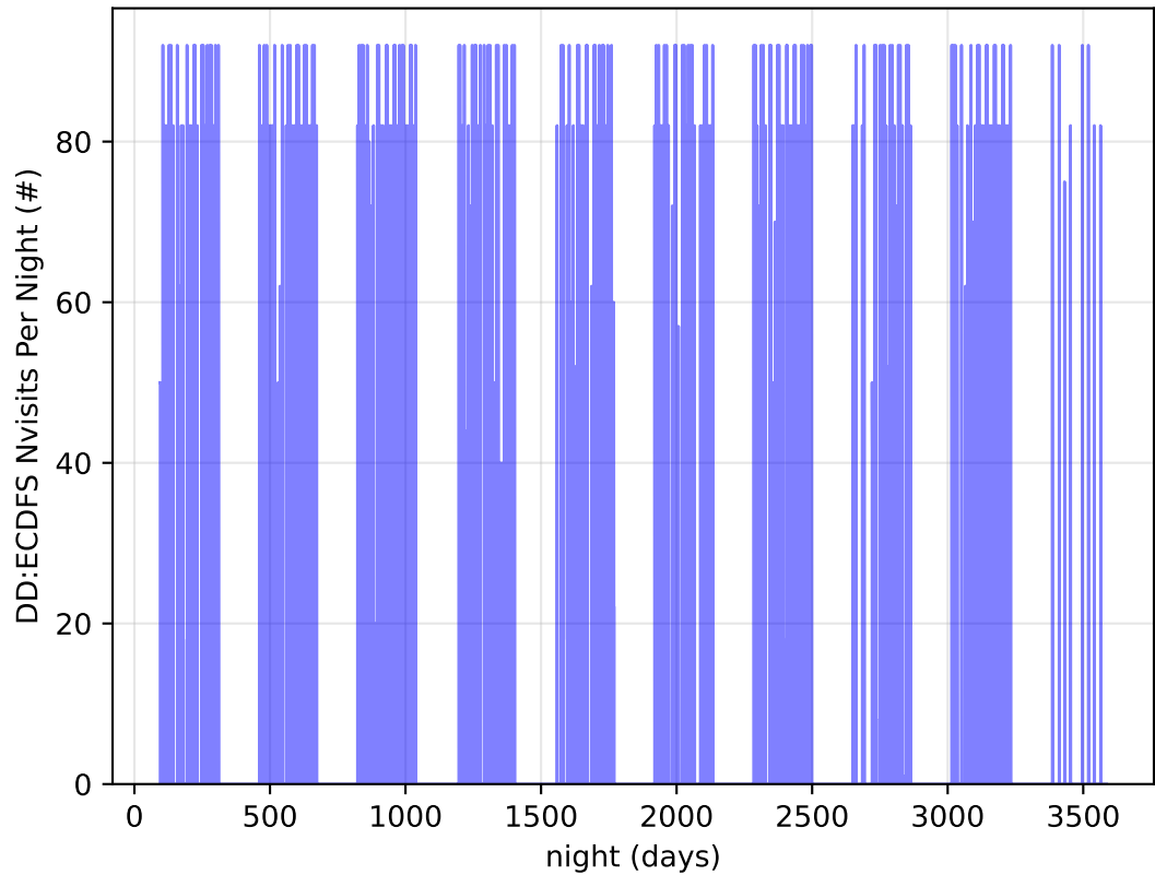
too_elab_2yr_r128_d2_griz_v3.4_10yrs all bands: DD:ECDFS Nvisits Per Night
