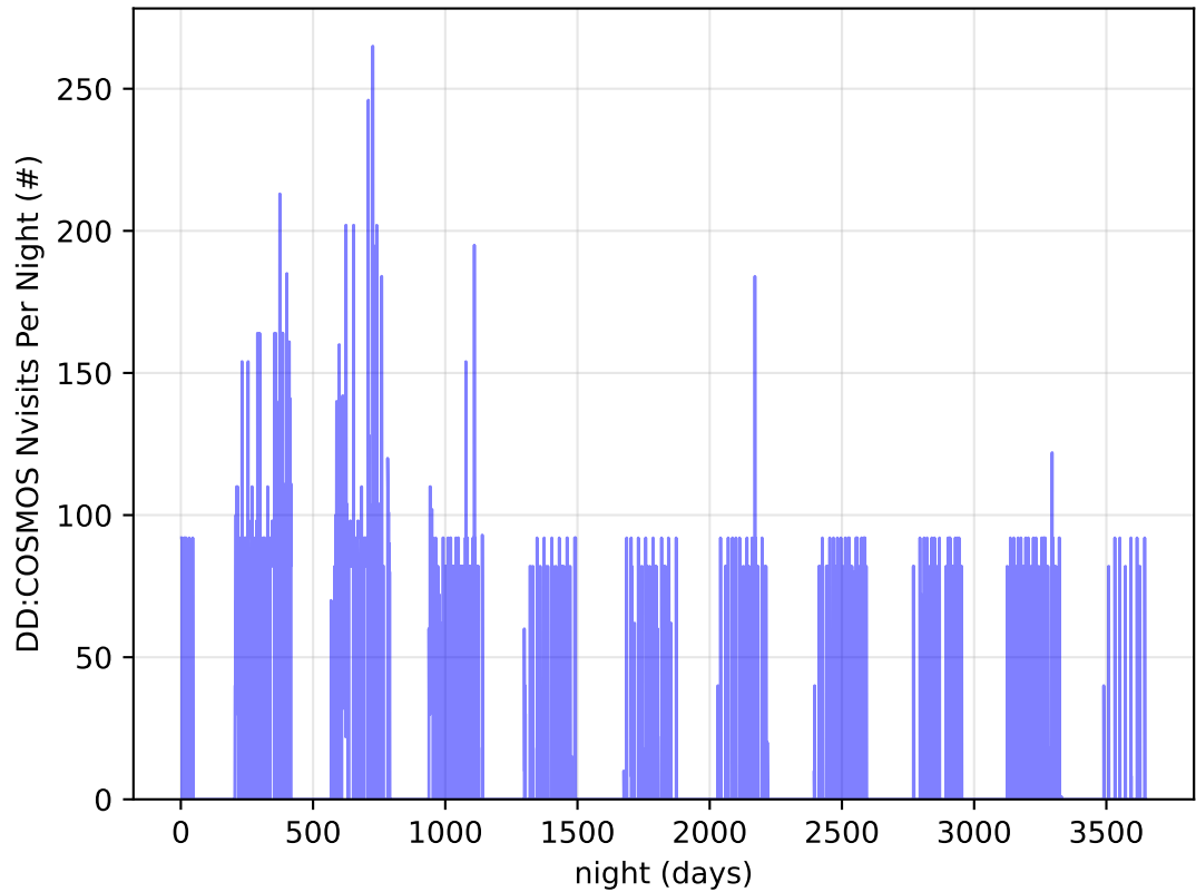
too_elab_2yr_r128_d2_griz_v3.4_10yrs all bands: DD:COSMOS Nvisits Per Night
