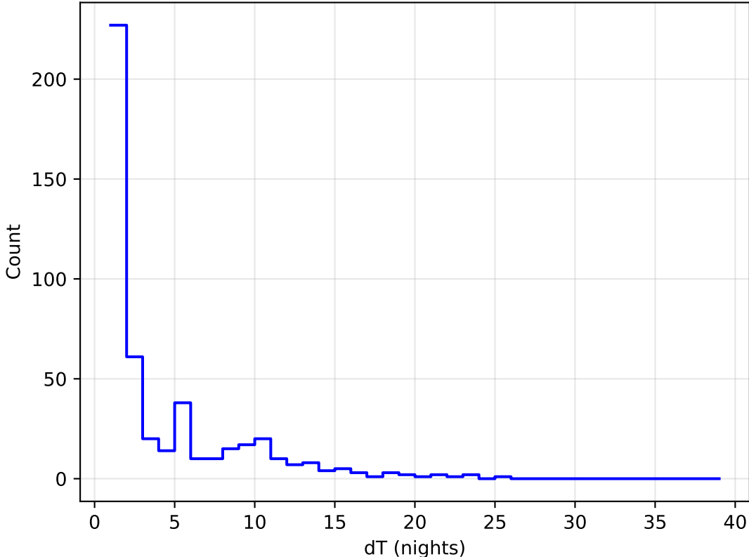
too_elab_2yr_r128_d2_griz_v3.4_10yrs all bands: DD: COSMOS Delta Nights Histogram
