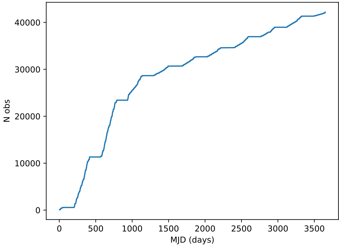
too_elab_2yr_r128_d2_griz_v3.4_10yrs all bands: DD:COSMOS Cumulative NVisits
