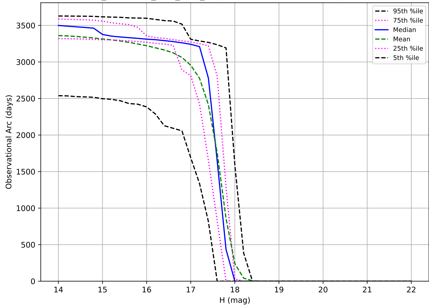
too_combined_s2.0_v3.4_10yrs: Observational Arc Length Trojan
