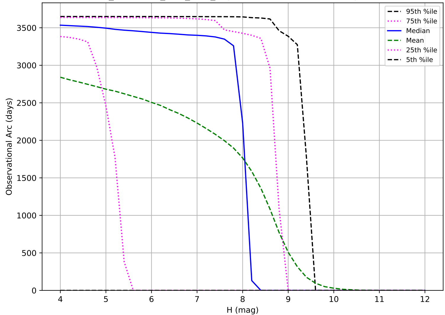
too_combined_s2.0_v3.4_10yrs: Observational Arc Length TNO
