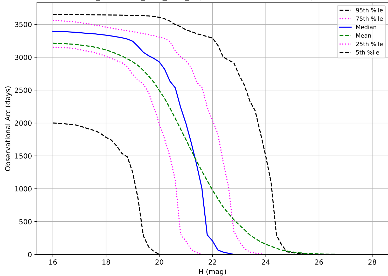
too_combined_s2.0_v3.4_10yrs: Observational Arc Length PHA
