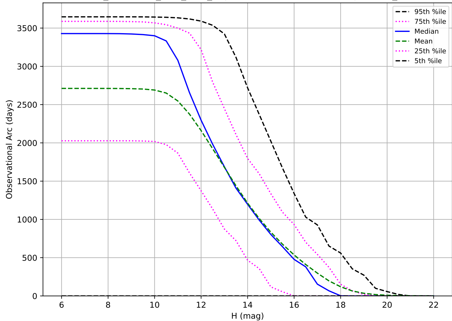
too_combined_s2.0_v3.4_10yrs: Observational Arc Length OCC_r5
