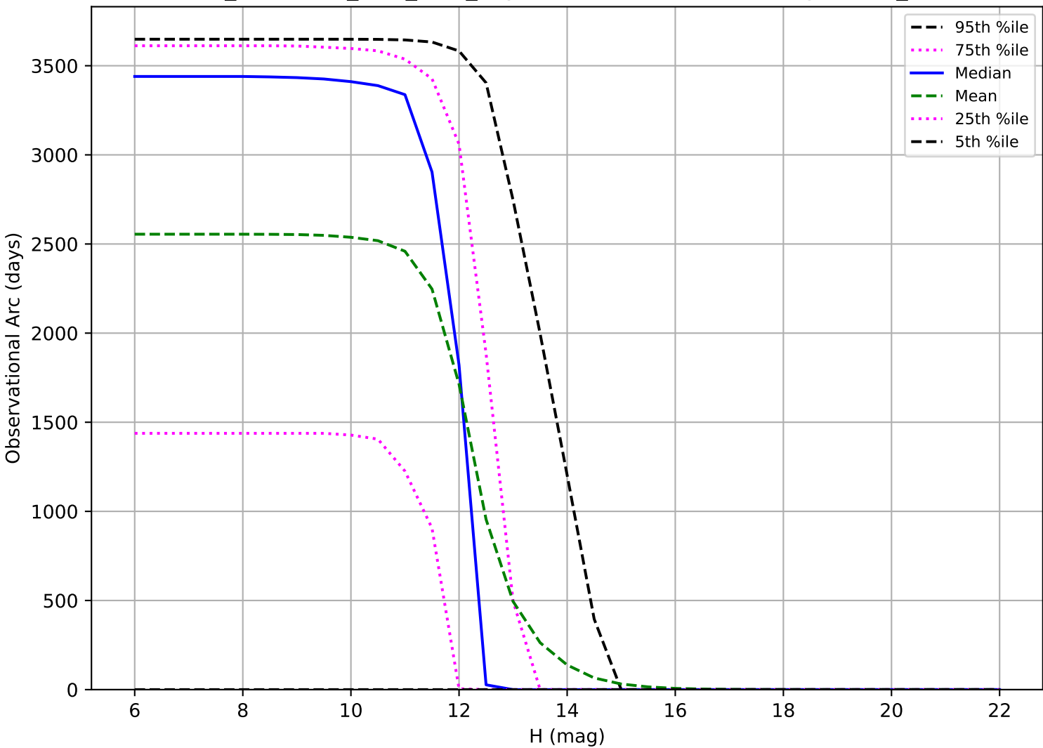
too_combined_s2.0_v3.4_10yrs: Observational Arc Length OCC_r20
