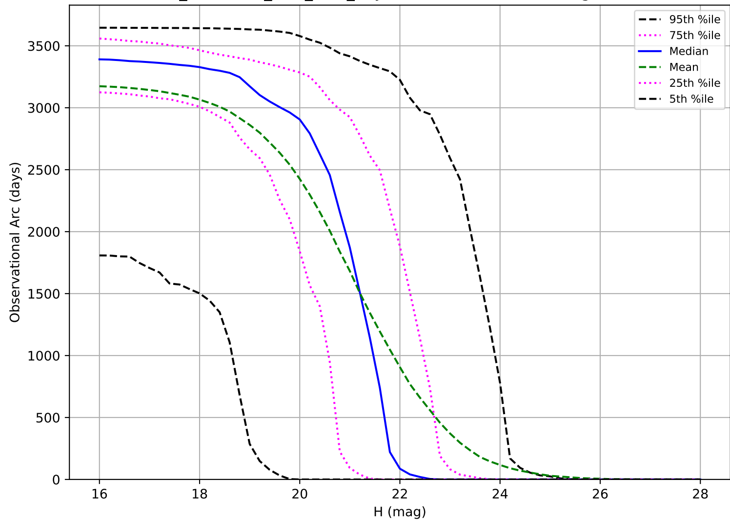
too_combined_s2.0_v3.4_10yrs: Observational Arc Length NEO
