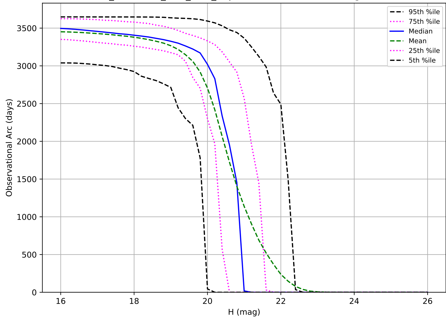
too_combined_s2.0_v3.4_10yrs: Observational Arc Length MBA
