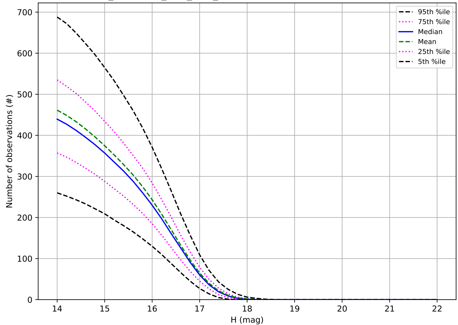
too_combined_s2.0_v3.4_10yrs: Number of observations Trojan
