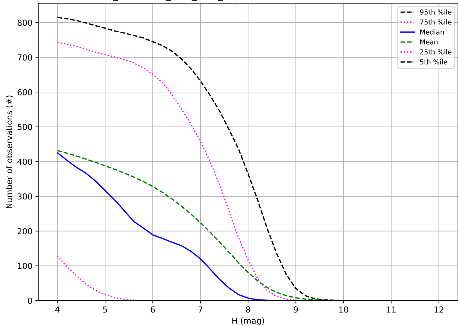
too_combined_s2.0_v3.4_10yrs: Number of observations TNO
