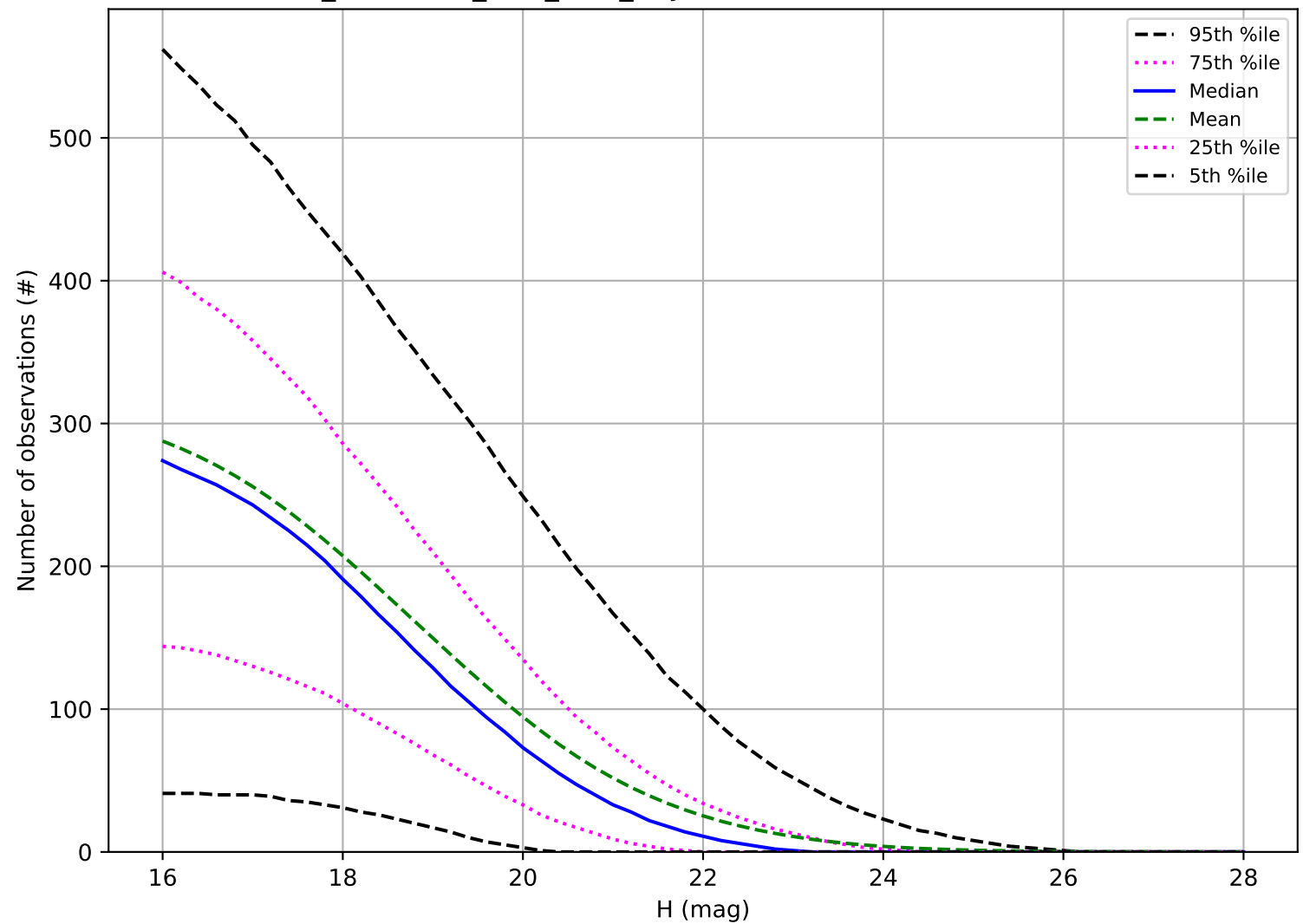
too_combined_s2.0_v3.4_10yrs: Number of observations PHA
