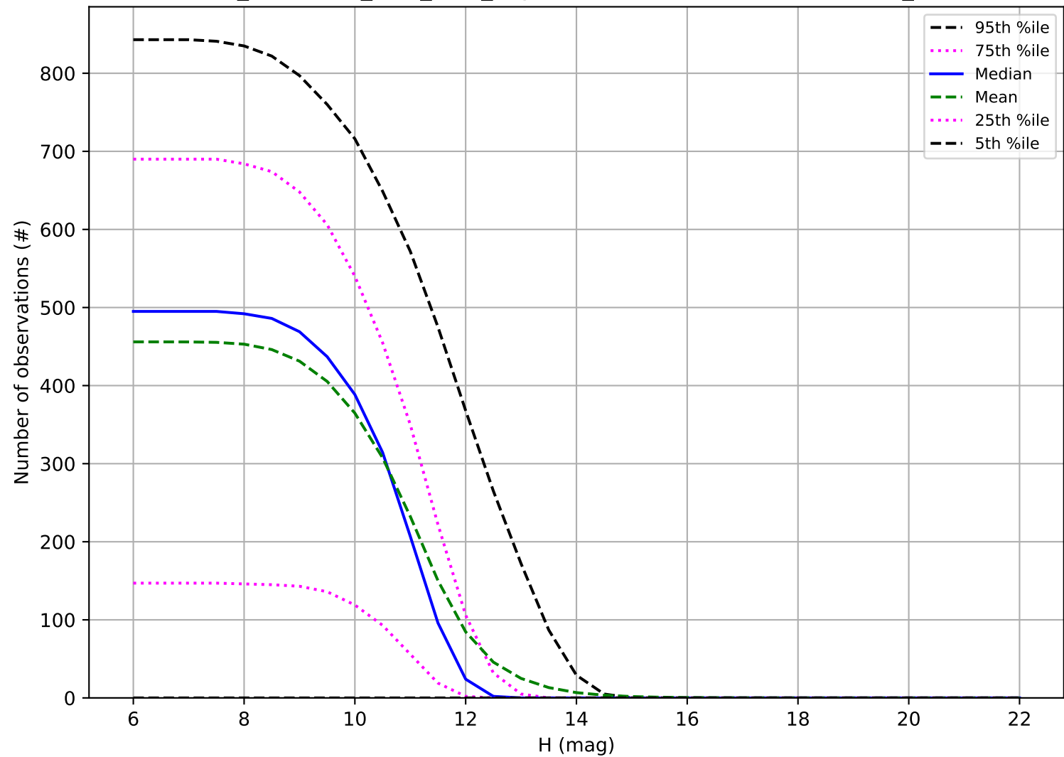
too_combined_s2.0_v3.4_10yrs: Number of observations OCC_r20
