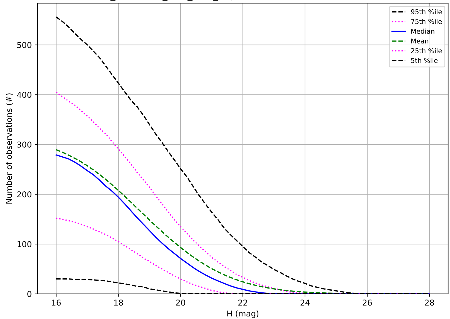
too_combined_s2.0_v3.4_10yrs: Number of observations NEO
