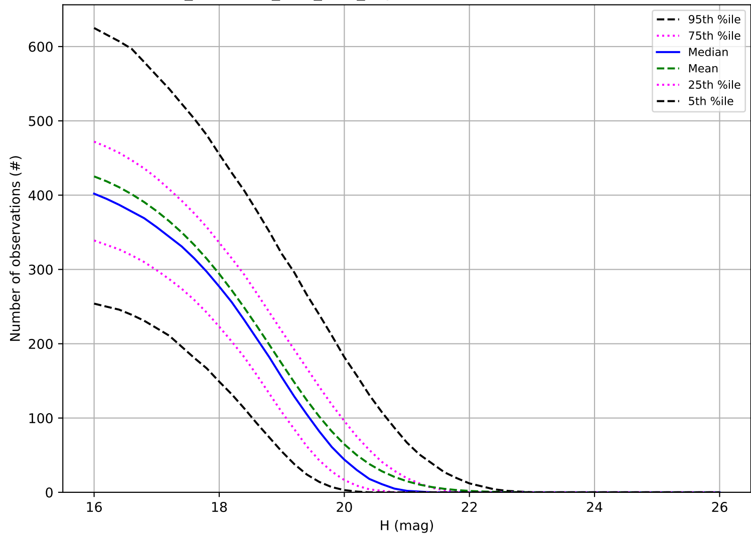
too_combined_s2.0_v3.4_10yrs: Number of observations MBA
