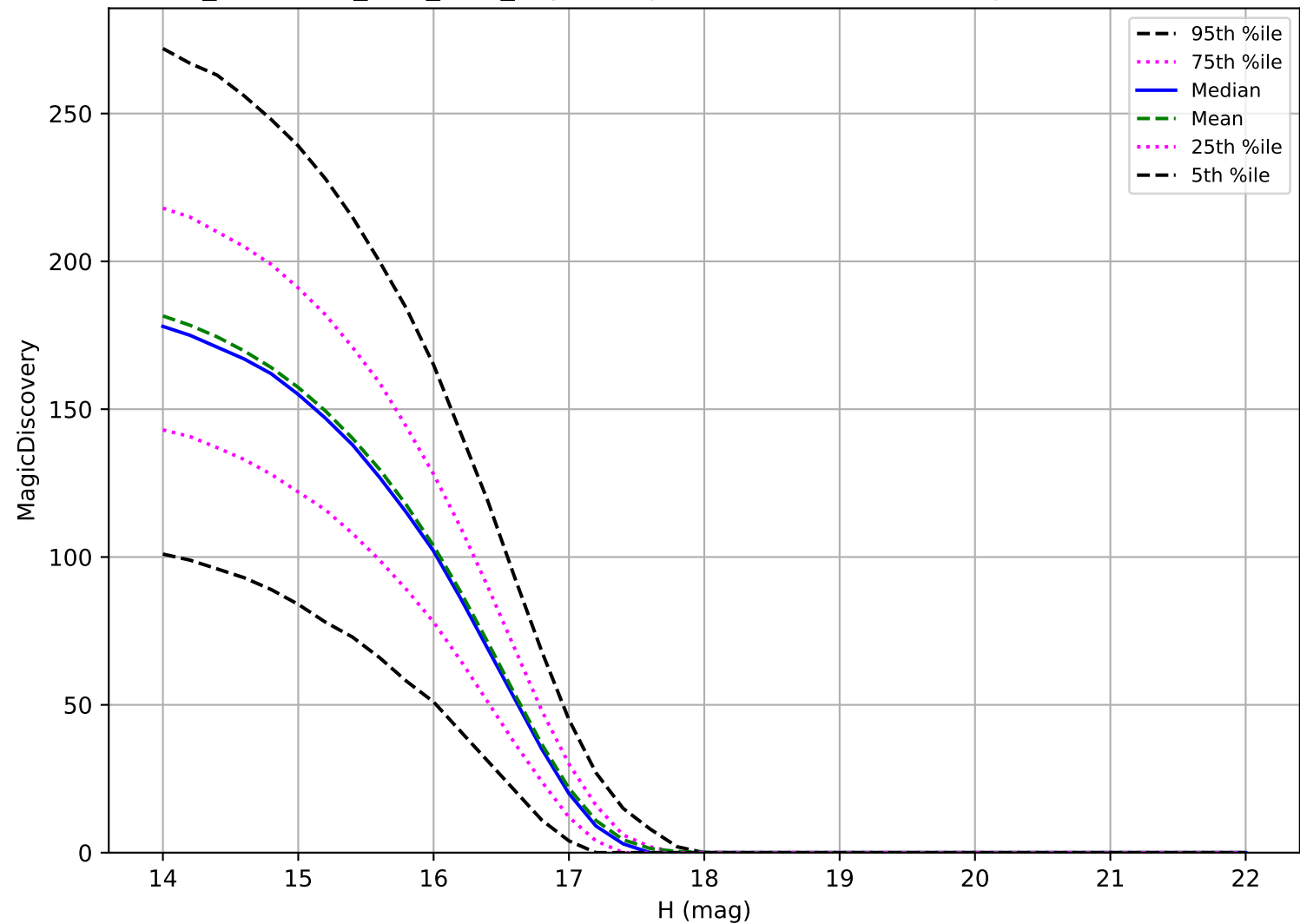
too_combined_s2.0_v3.4_10yrs: Trojan 6 detections in 60 nights detection loss
