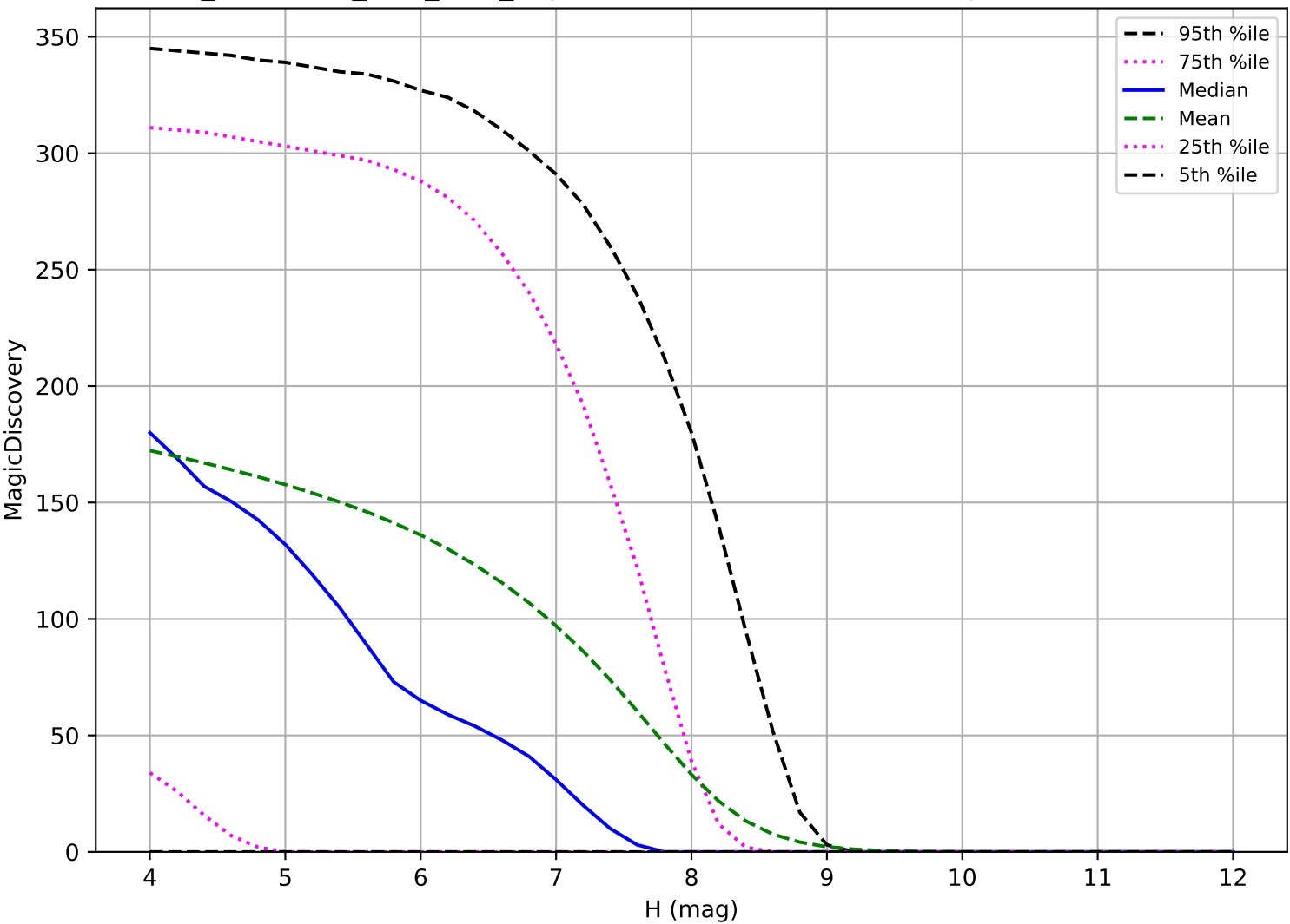
too_combined_s2.0_v3.4_10yrs: TNO 6 detections in 60 nights detection loss
