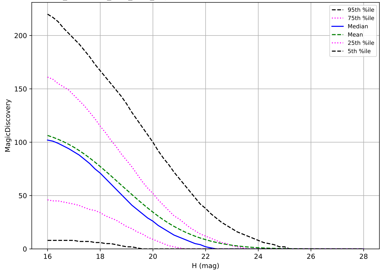
too_combined_s2.0_v3.4_10yrs: PHA 6 detections in 60 nights detection loss
