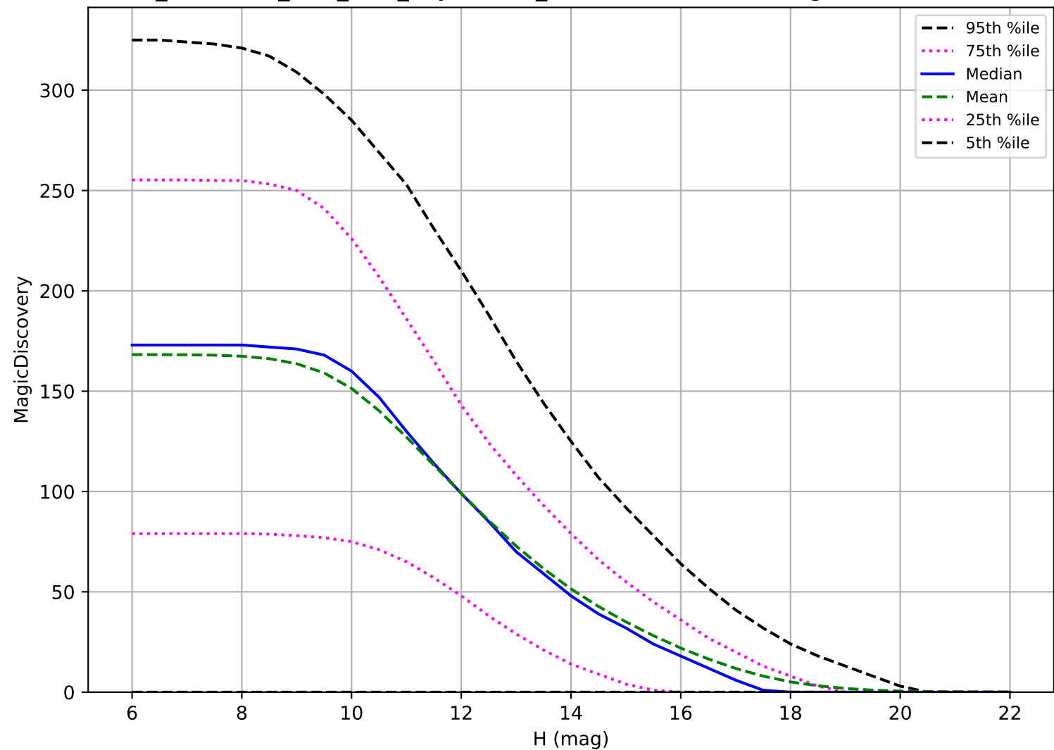
too_combined_s2.0_v3.4_10yrs: OCC_r5 6 detections in 60 nights detection loss
