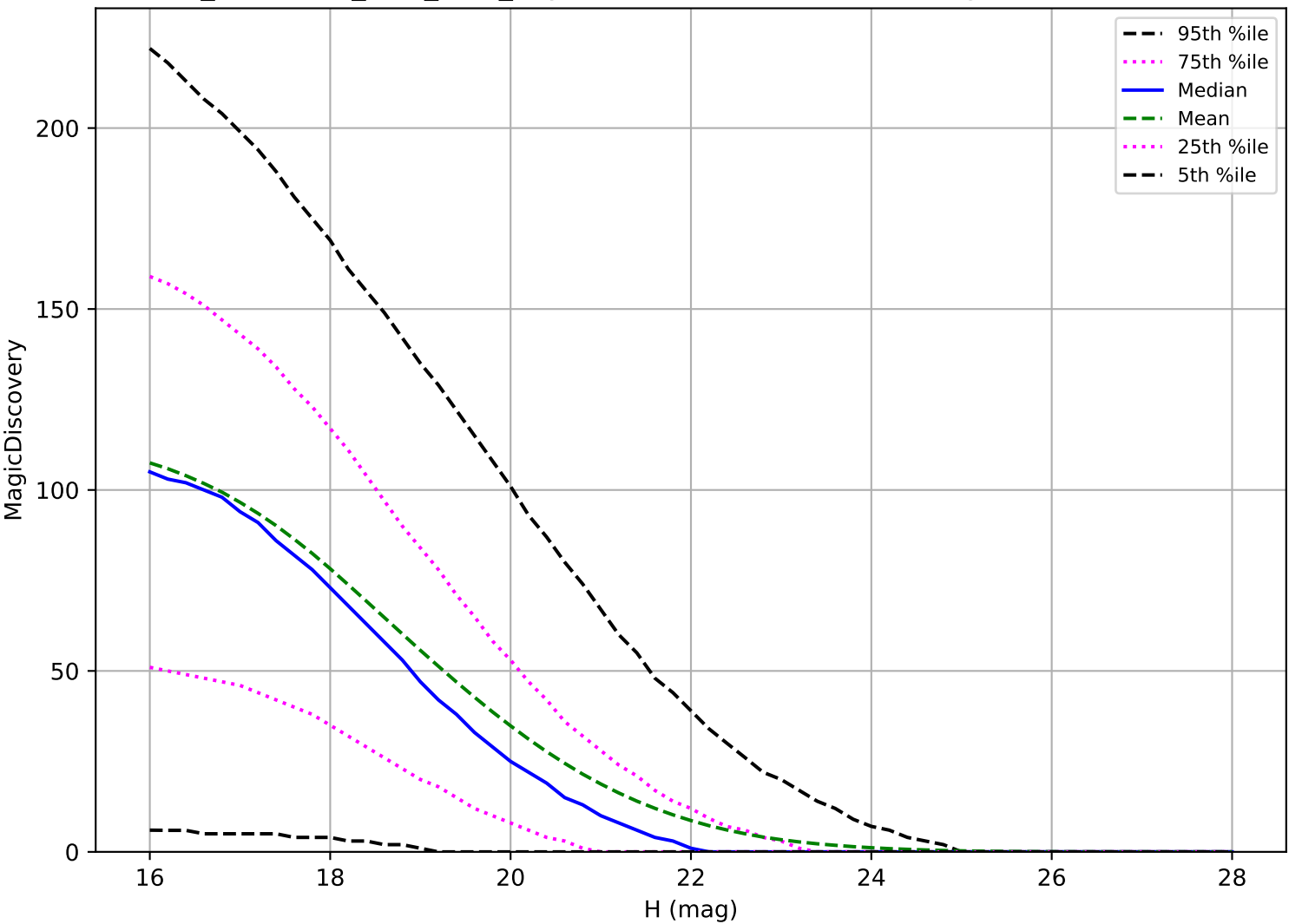
too_combined_s2.0_v3.4_10yrs: NEO 6 detections in 60 nights detection loss
