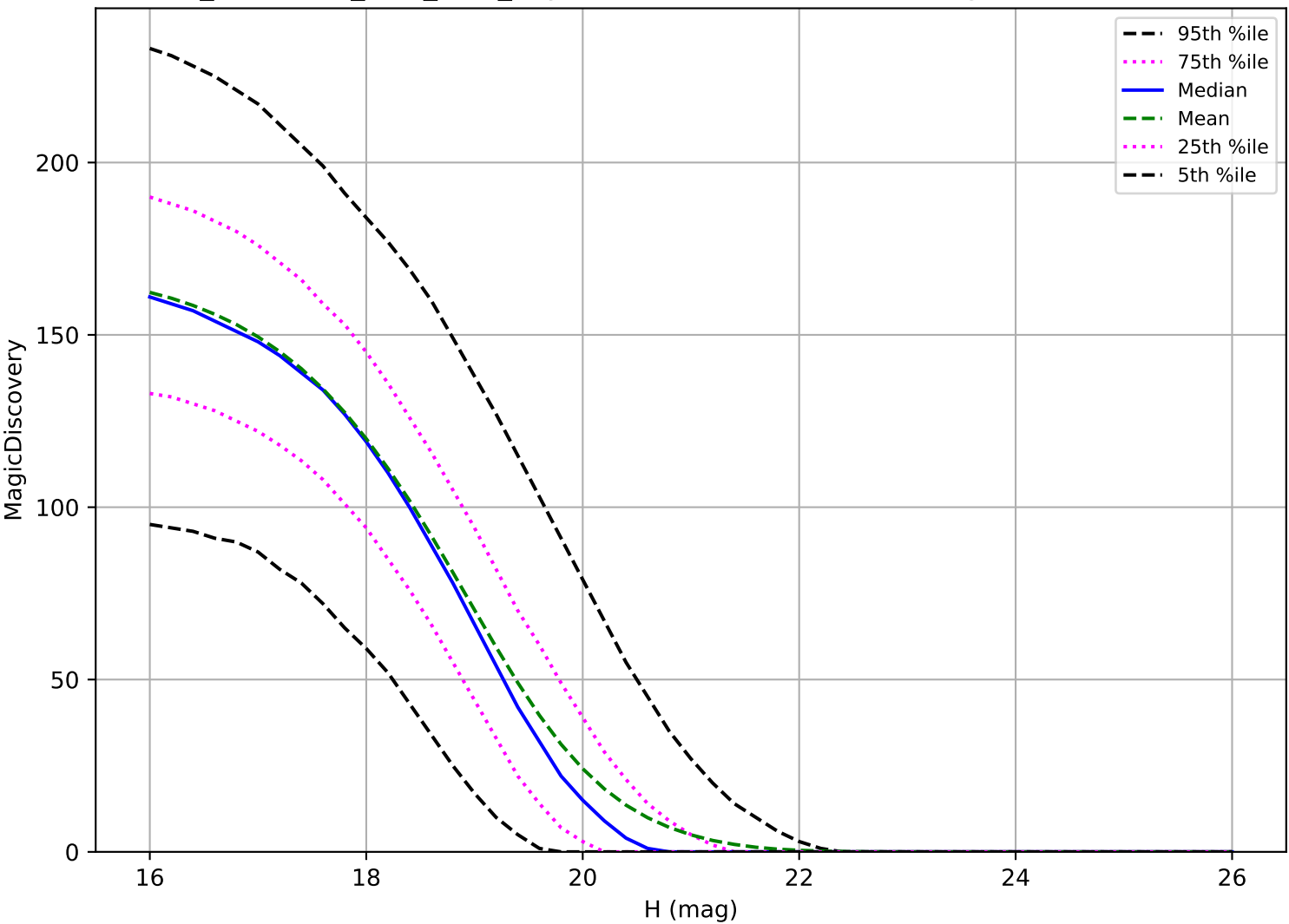
too_combined_s2.0_v3.4_10yrs: MBA 6 detections in 60 nights detection loss
