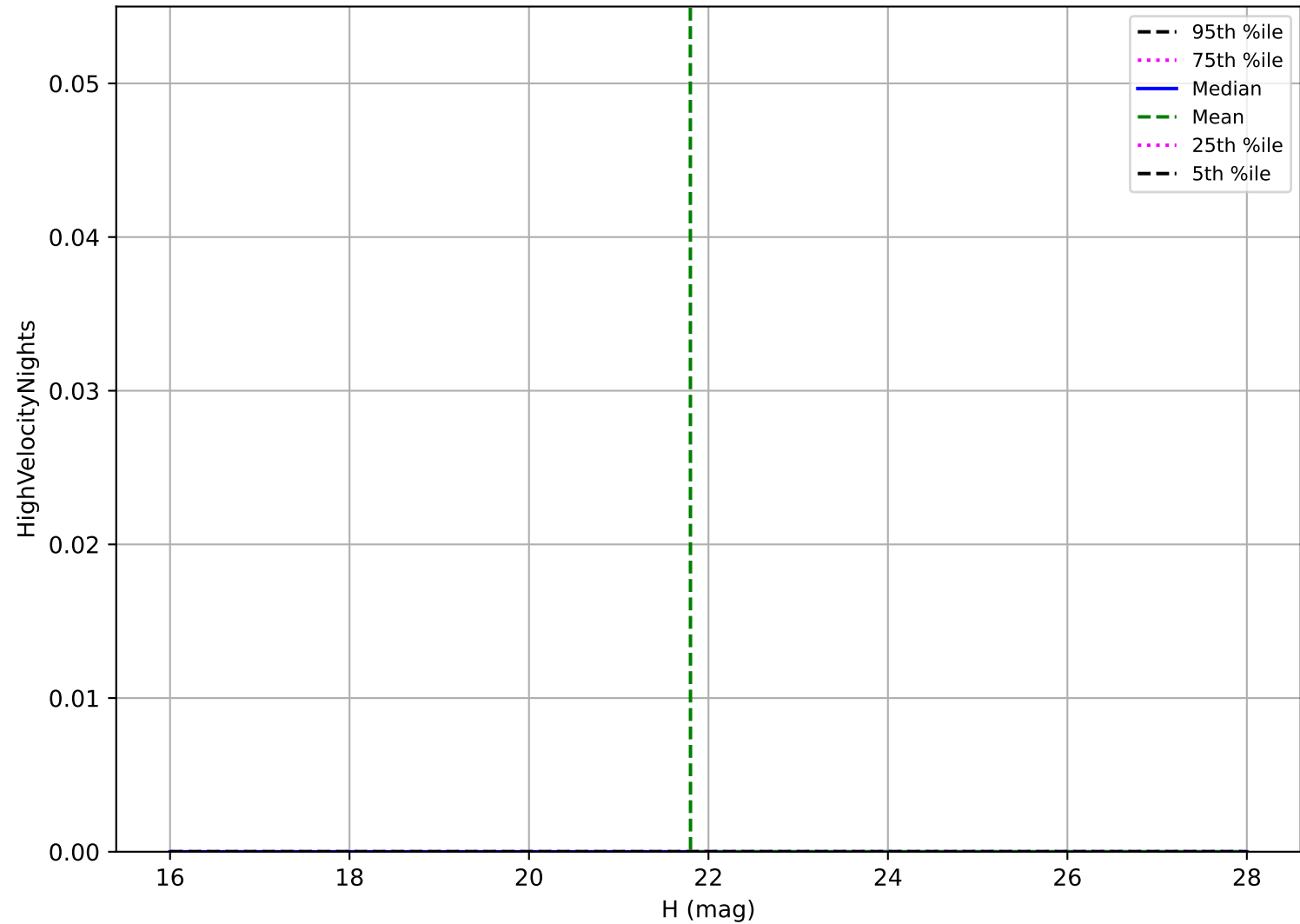
too_combined_s2.0_v3.4_10yrs: Vatira High velocity pair detection loss
