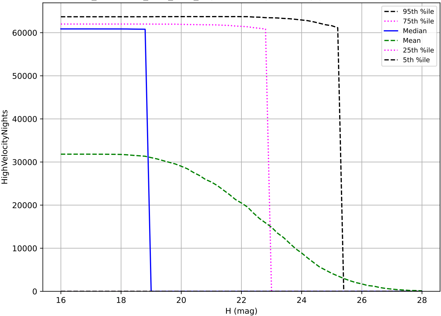
too_combined_s2.0_v3.4_10yrs: PHA High velocity pair detection loss
