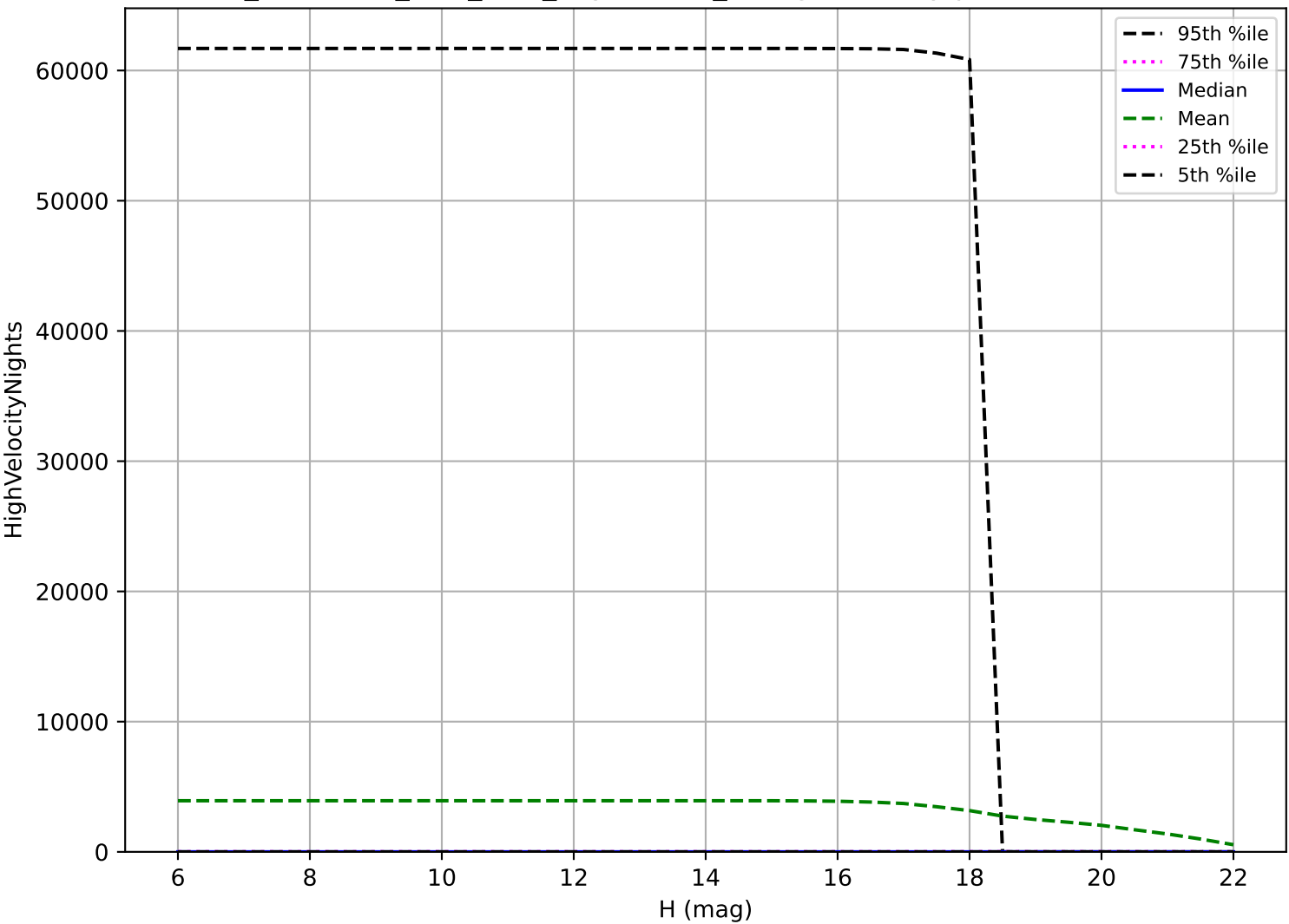
too_combined_s2.0_v3.4_10yrs: OCC_r5 High velocity pair detection loss
