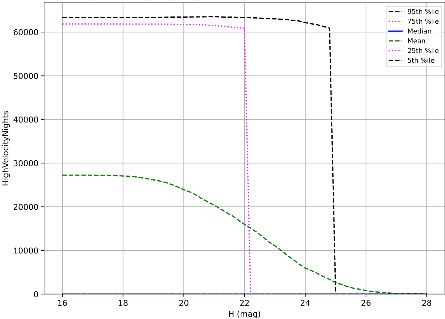
too_combined_s2.0_v3.4_10yrs: NEO High velocity pair detection loss
