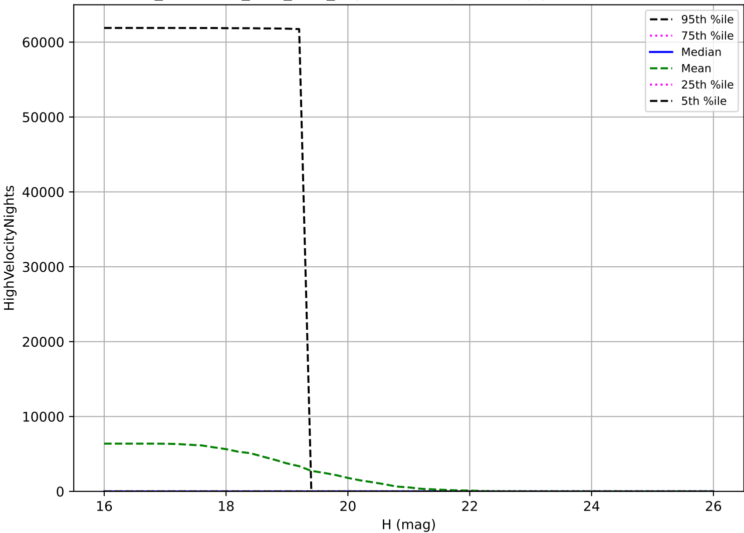
too_combined_s2.0_v3.4_10yrs: MBA High velocity pair detection loss
