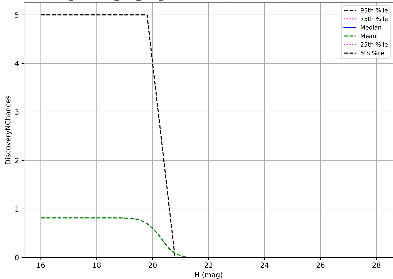
too_combined_s2.0_v3.4_10yrs: Vatira 3 pairs in 15 nights detection loss
