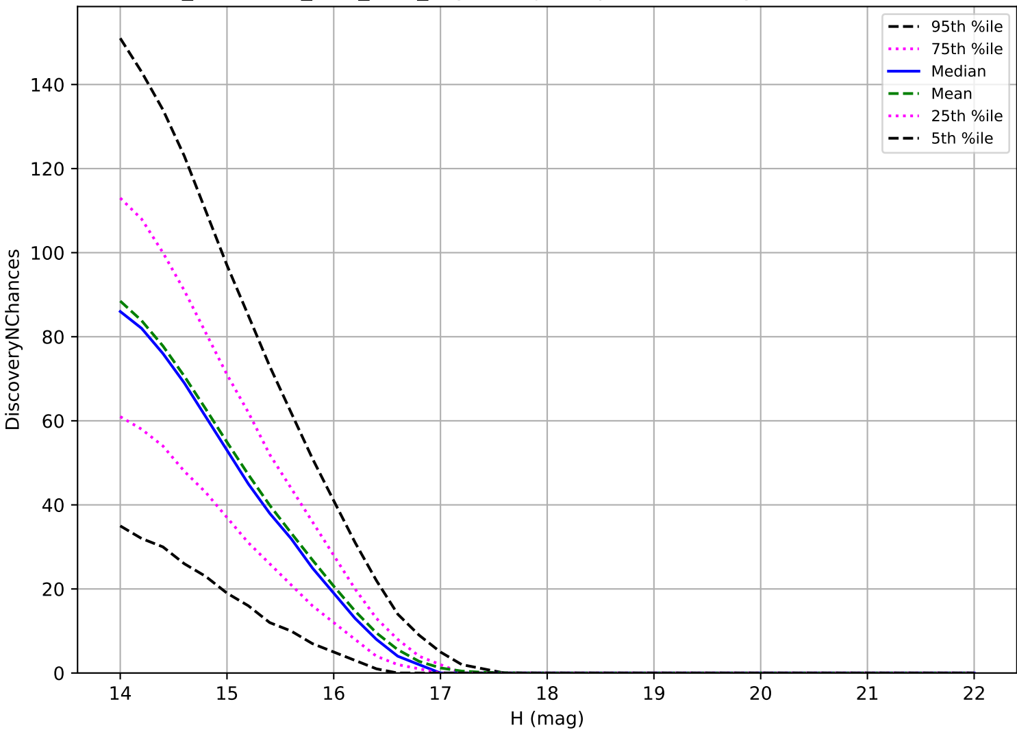
too_combined_s2.0_v3.4_10yrs: Trojan 3 pairs in 15 nights detection loss
