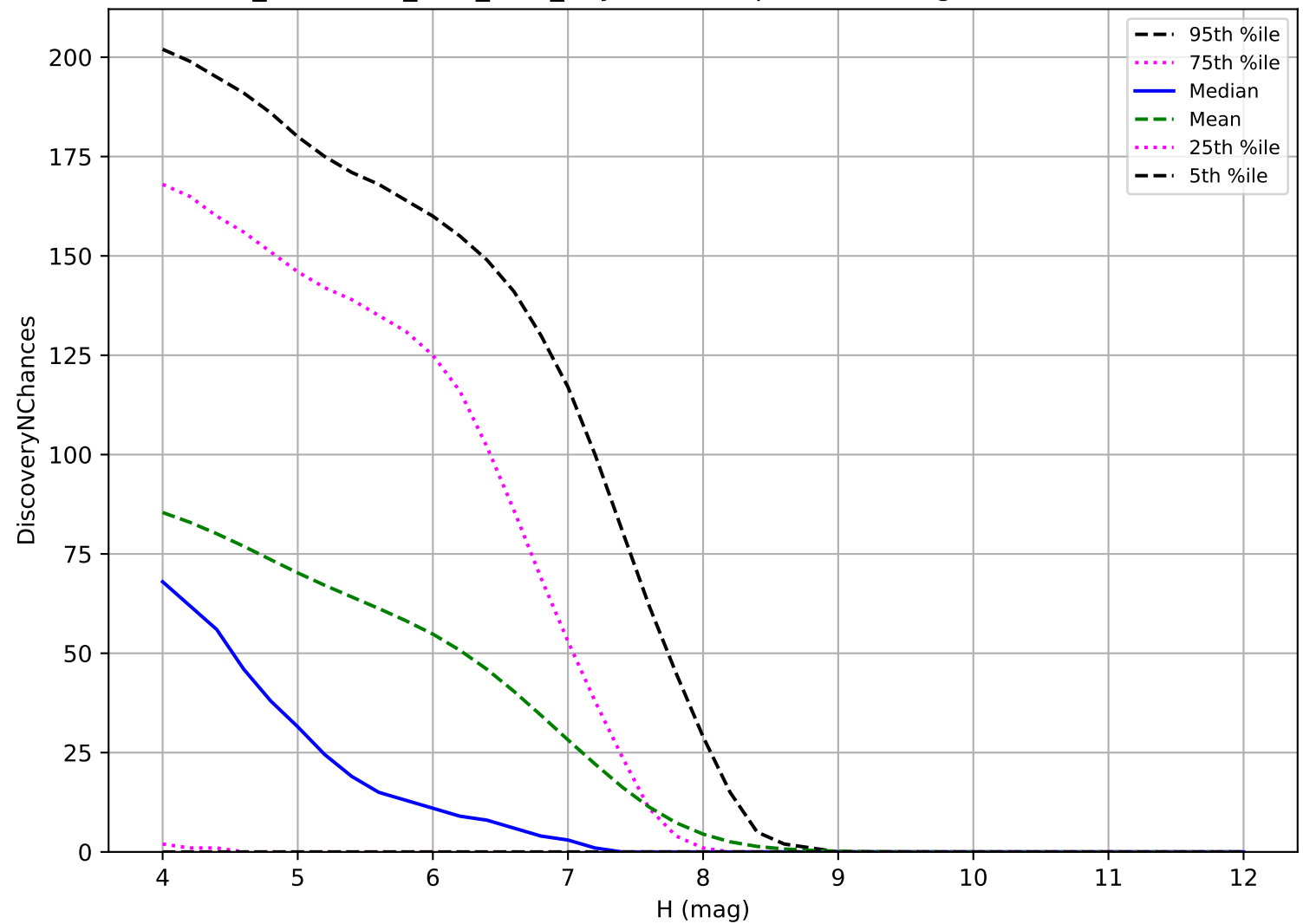
too_combined_s2.0_v3.4_10yrs: TNO 3 pairs in 15 nights detection loss
